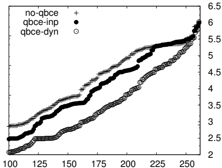
Fig. 3. Related to Table 1: sorted numbers of backtracks ( \log_{10} scale y-axis) by DepQBF, qbce-inp, and qbce-dyn on 262 instances solved by all three (x-axis).
